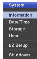
Figure 8 — System menu.
