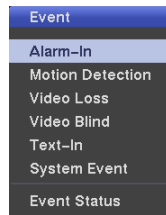
Figure 26 — Event menu.
