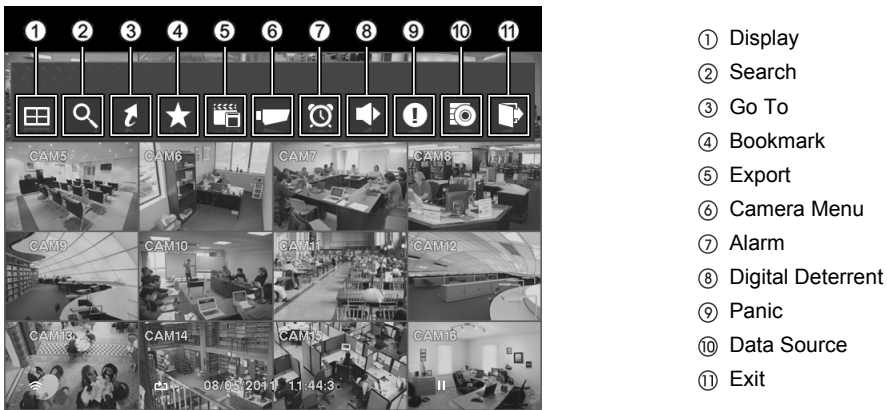
Figure 74 — Search menu.
