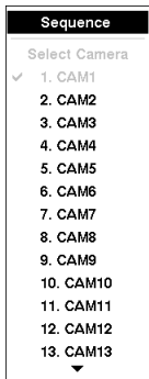
Figure 72 — Sequence menu.
