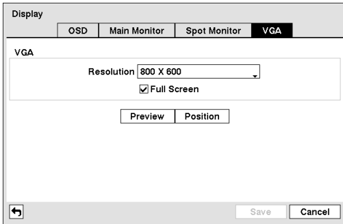
Figure 67 — VGA screen.
