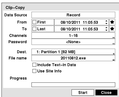
Figure 81 — Clip-Copy screen.
